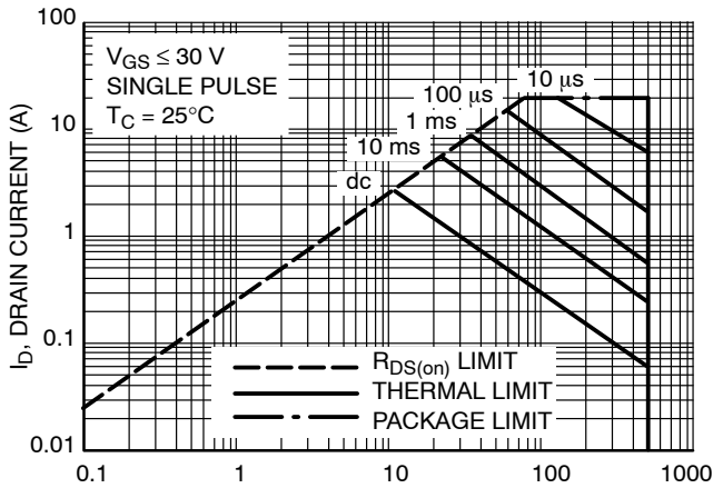
Figure 12. Maximum Rated Forward Biased Safe Operating Area NDF05N50Z
